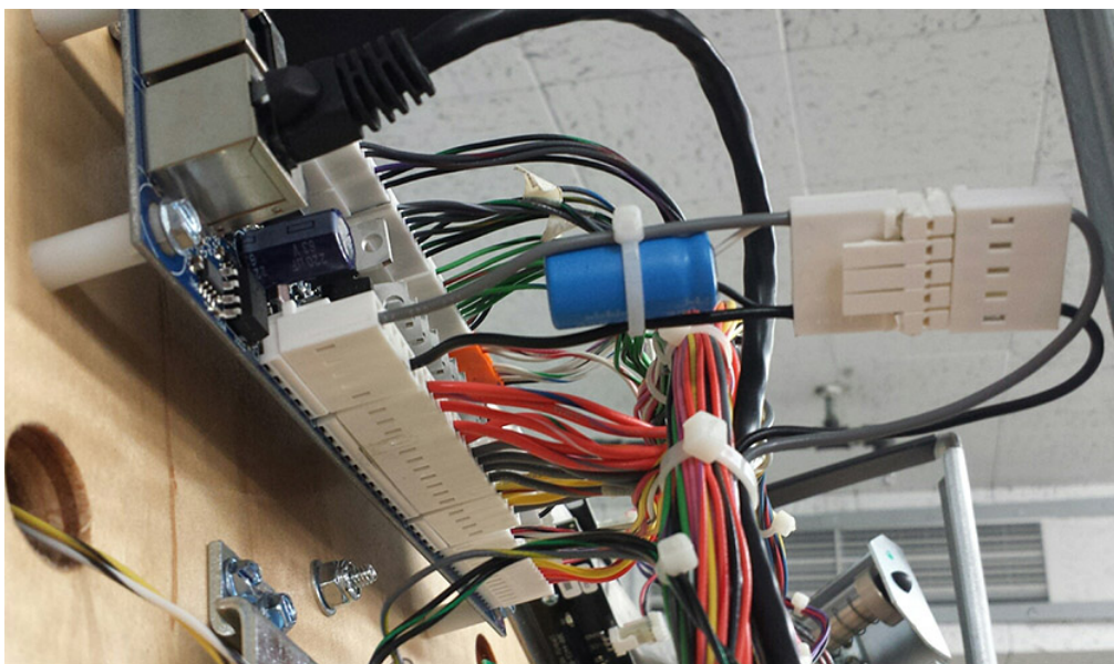
Ex: Capacitor Kit installed on Node 8
