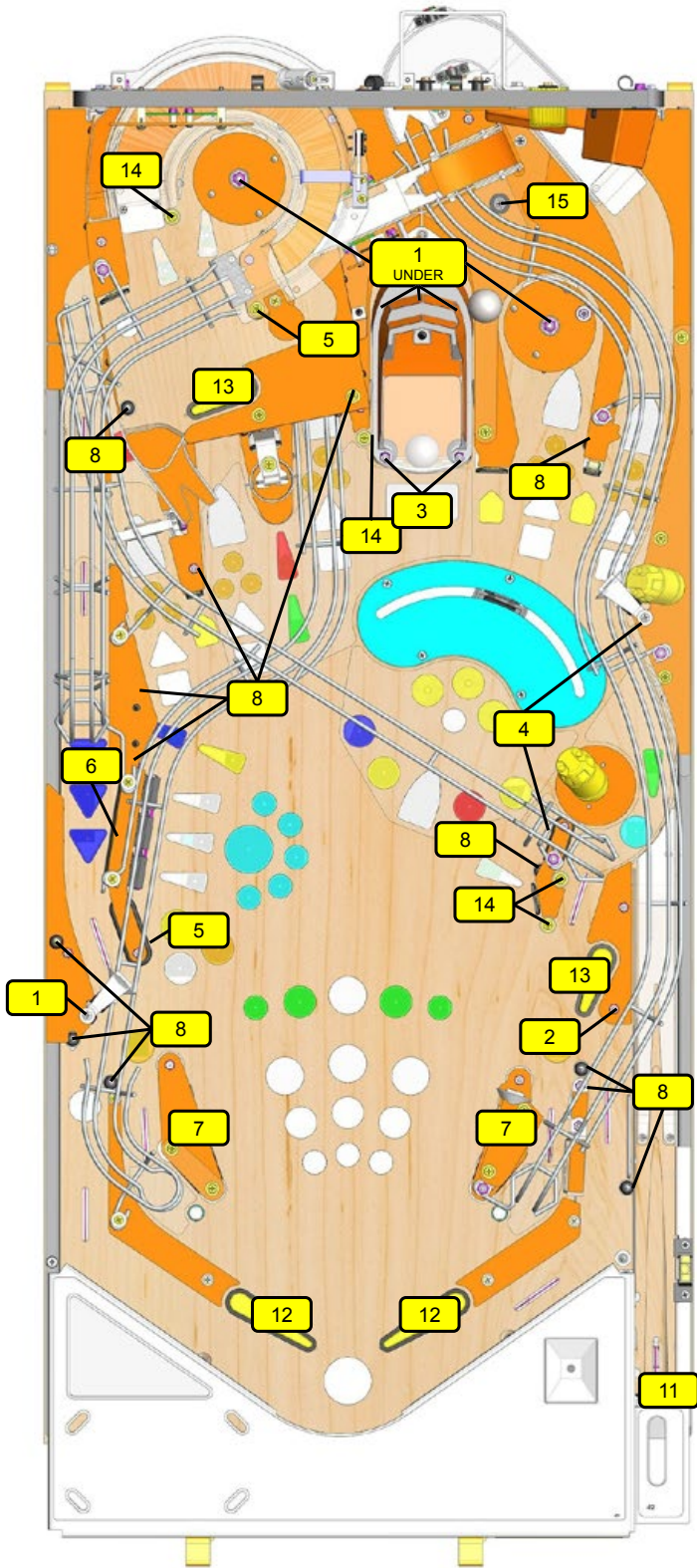
Figure 5.1.1. Rubber o-ring part locations
