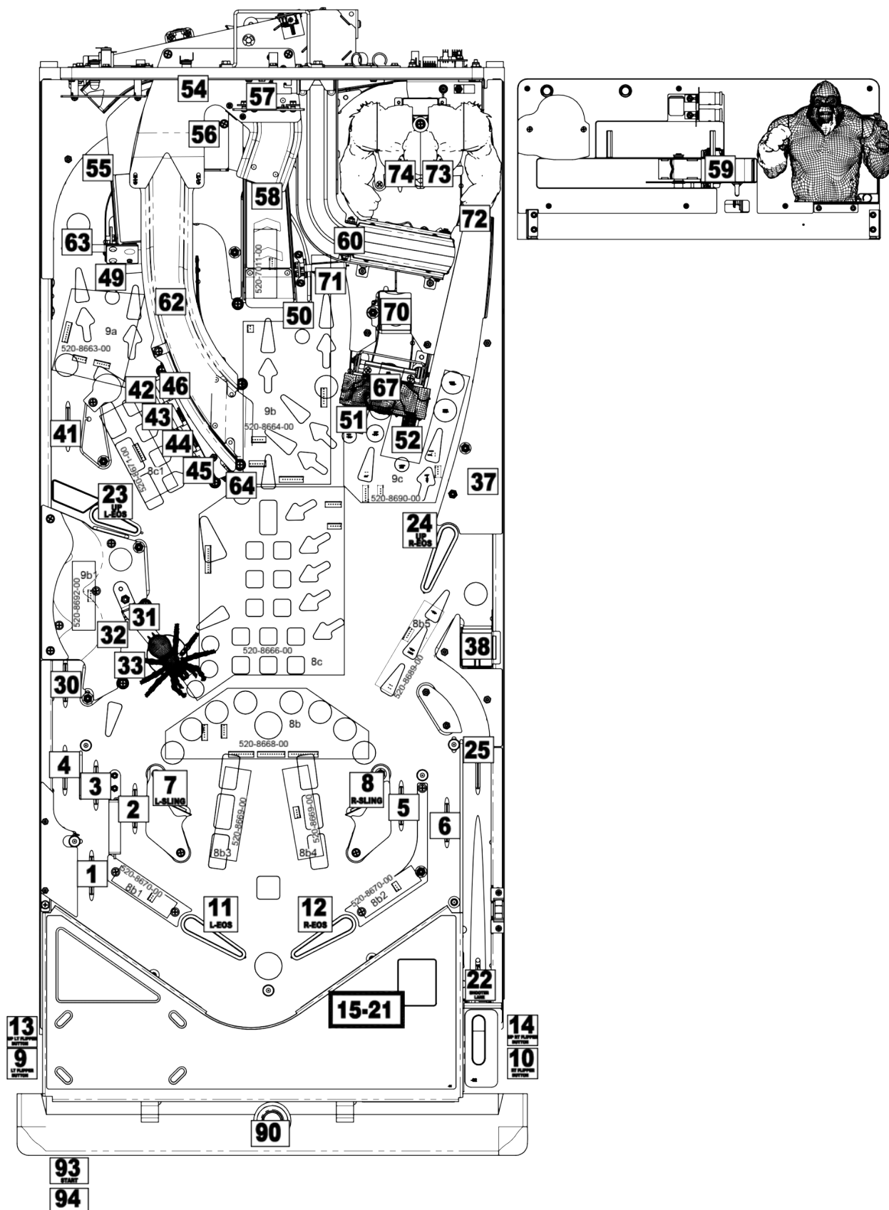
Figure 3.3.1. Playfield switch locations (top view).
